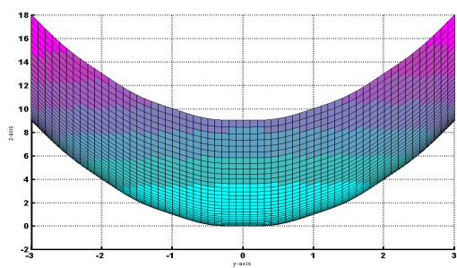
Figure 3: yz -view of Figure 1.
