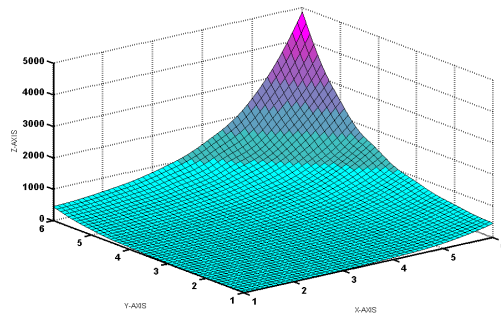
Figure 4: Convex rational bi-cubic surface.
