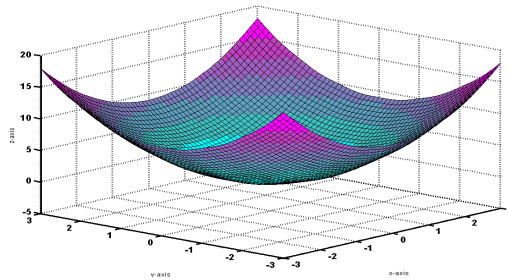
Figure 1: Convex rational bi-cubic surface.
