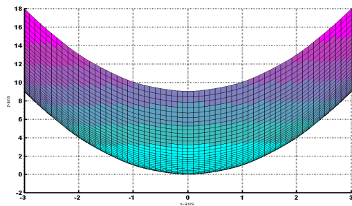
Figure 2: xz -view of Figure 1.
