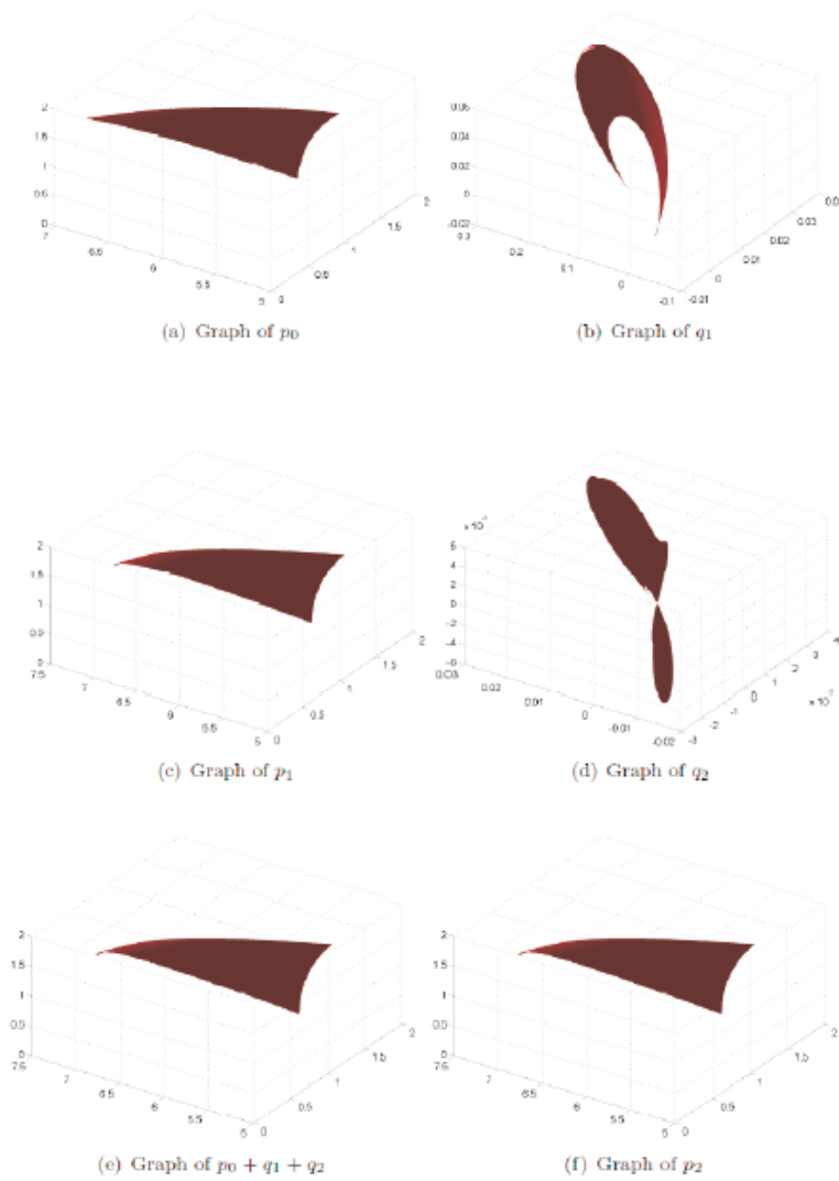
Figure 3. Decomposition of p_2 .
