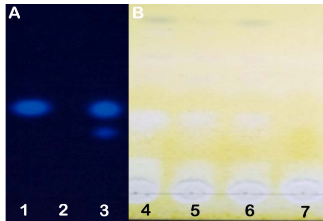
Figure 1. Thin-layer chromatography analysis of AFB 1 (A) and CPA (B) production in A. flavus strains: 1A) AFB 1 standard, 2A) non-toxicogenic A. flavus PICC-AF69, 3A) toxicogenic A. flavus PICC-AF98, 4B) CPA standard, 5B) toxicogenic A. flavus PICC-AF69, 6B) non-toxicogenic A. flavus PICC-AF98 and 7B) A. flavus CMI 93803.
