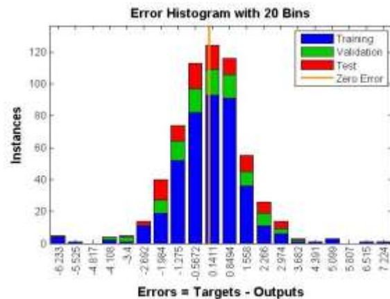
Fig. 6 Diagram of the network histogram error
