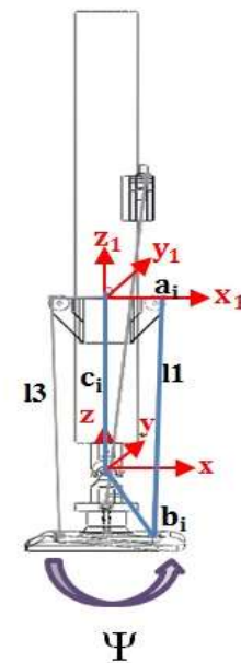
Fig. 3 Position vector of points in the mechanism of cable robot from the front view
