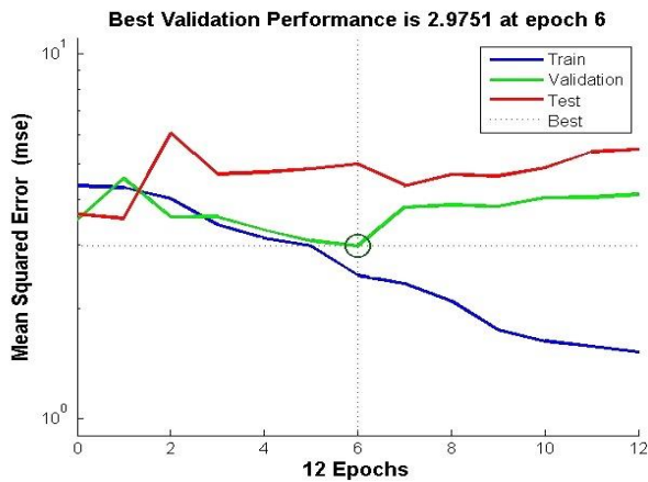
Fig. 8 Validation for the best operation of network
