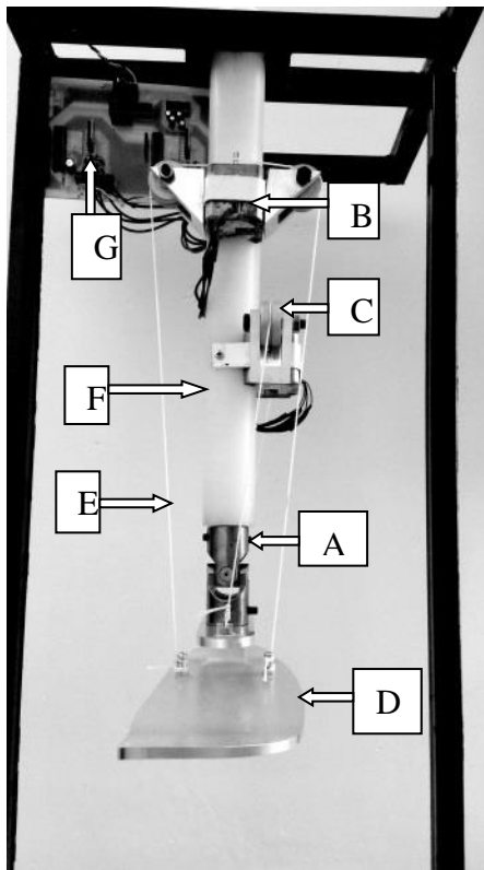
Fig. 9 Constituent components of the artificial limb or organ
