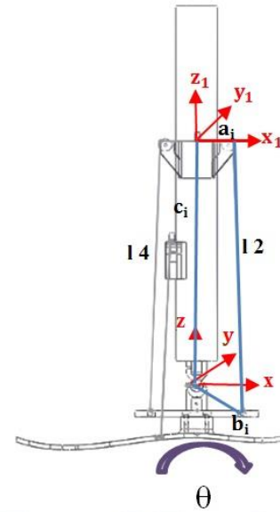
Fig. 2 Position vector of points in mechanism of cable robot from the side view
