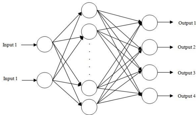
Fig. 4 Schematic of a neural network
