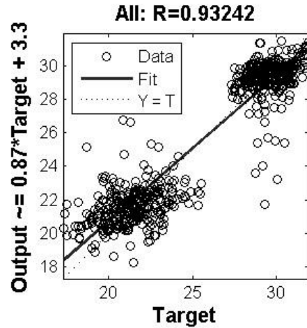
Fig. 5 Output of the network instruction percent
