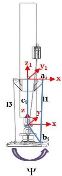
Fig. 3 Position vector of points in the mechanism of cable robot from the front view
