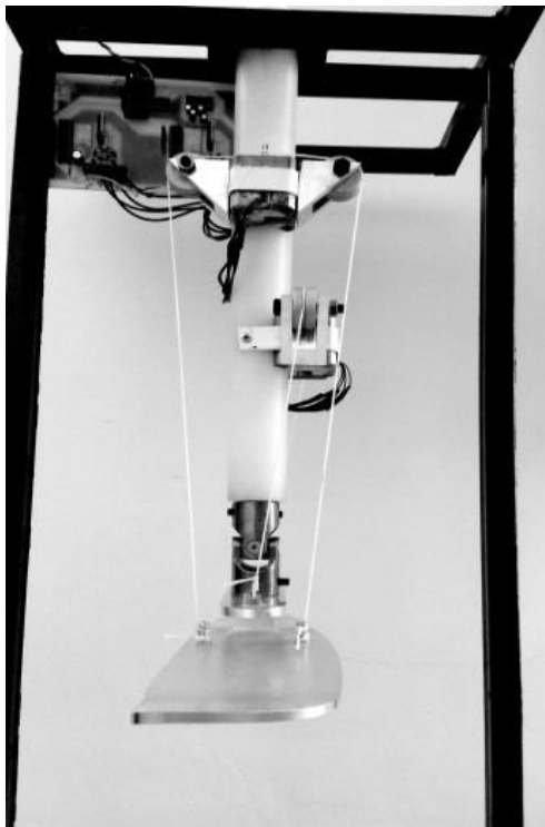
Fig. 10 Laboratory sample of artificial limb or organ before rotation
