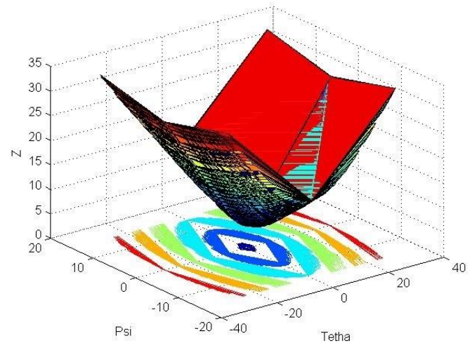
Fig. 12 The obtained workspace according to the kinematic relations
