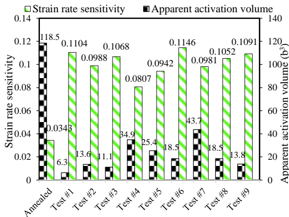
Fig. 4 Strain rate sensitivity and apparent activation volume for the products of Exp-ECAE experiments conducted based on Table 1.
