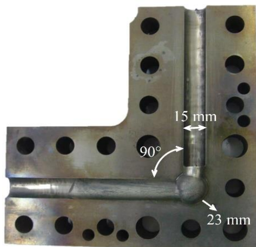
Fig. 1 One half of the Exp-ECAE die and the partially deformed component
