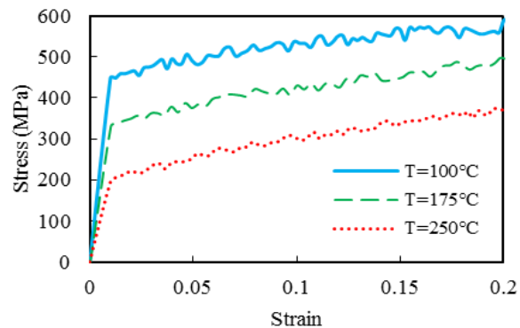
Fig. 5 The stress-strain behavior recorded at strain rate of 2000 s^{-1} for the billets processed with a ram velocity of 7 mm/min and at different temperatures.
