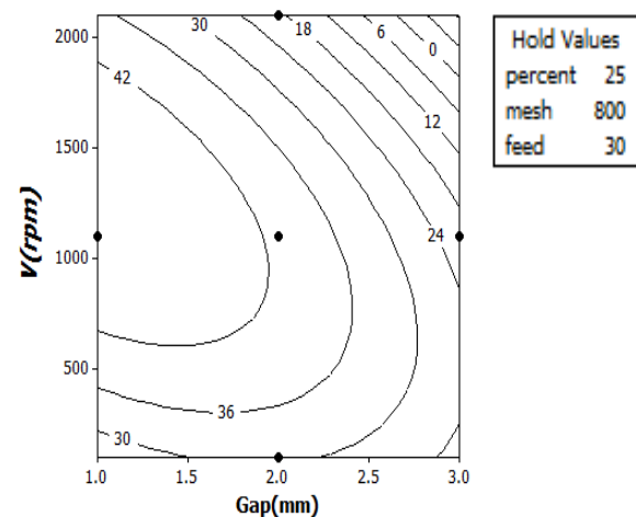
Fig. 12 Interaction of gap and rotational speed
