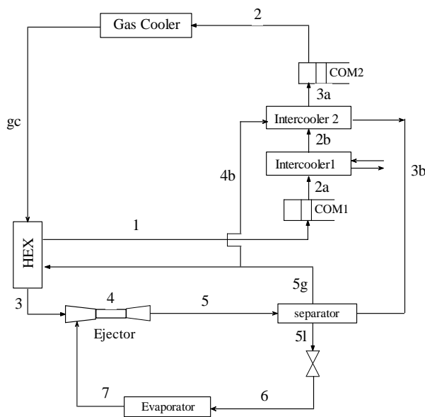
Fig. 3 Schematic of new multi-inter-cooling two-stage TRCC cycle with ejector and internal heat exchanger
