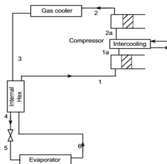
Fig. 1 Schematic of internal heat exchanger two-stage TRCC cycle (IHEC)
