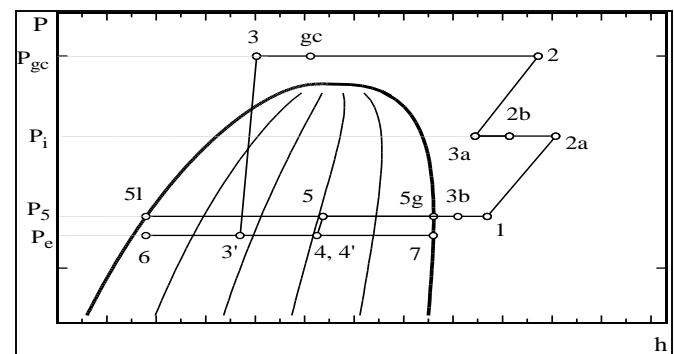
Fig. 4 P-h diagram of new multi-inter-cooling two-stage TRCC cycle with ejector and internal heat exchanger
