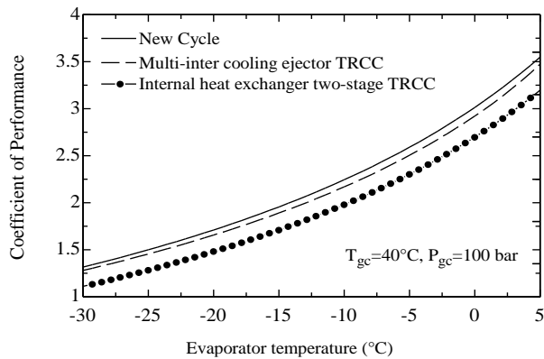
Fig. 7 The COP value of three cycles versus evaporator outlet temperature
