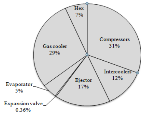
Fig. 10 Exergy destruction rate in each component of the new cycle
