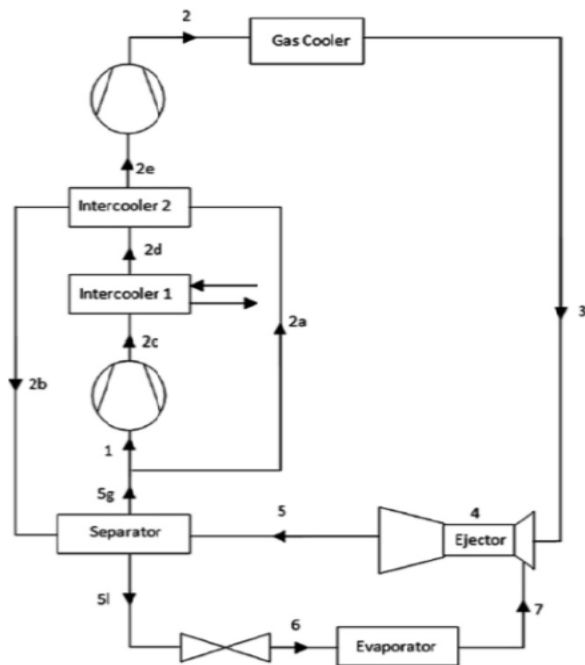
Fig. 2 Schematic of multi-inter-cooling two-stage TRCC cycle with ejector expansion device (MIERC)
