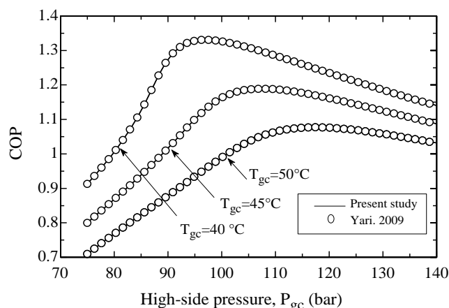
Fig. 5 Comparison of the present simulation result with the Yari [7] Results.
