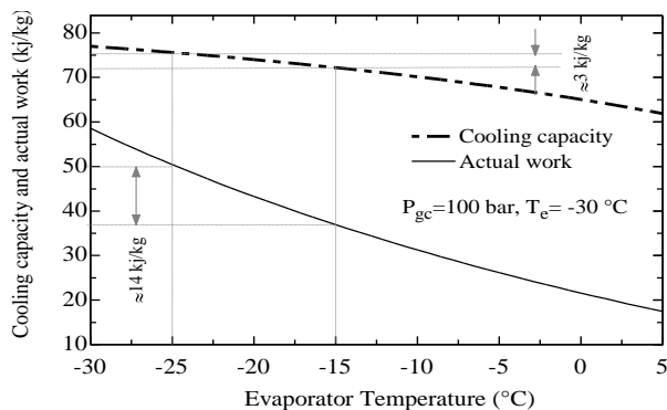
Fig. 8 The cooling capacity and actual work of the cycle value of the new cycle versus evaporator outlet temperature
