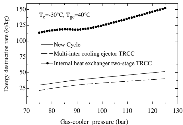
Fig. 11 Exergy destruction rate value of three cycles versus gas cooler pressure
