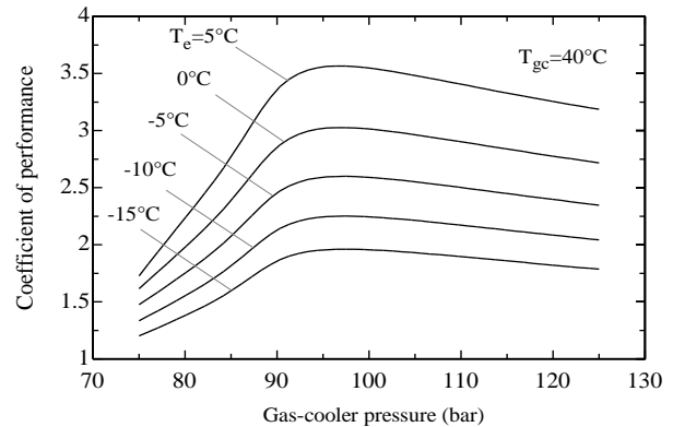
Fig. 9 The COP value of the new cycle versus gas cooler pressure under different evaporator outlet temperature
