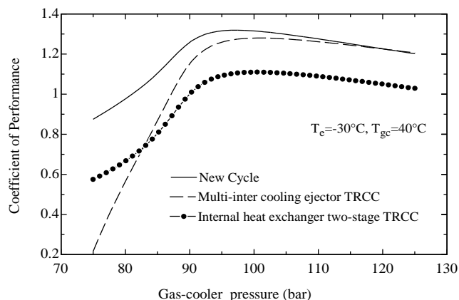
Fig. 6 The COP value of three cycles versus gas cooler pressure
