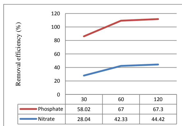
Figure 7c. Effect of contact time on the removal of nitrate and phosphate at adsorbent dose 2 gr/l and mixing speed 100 rpm
