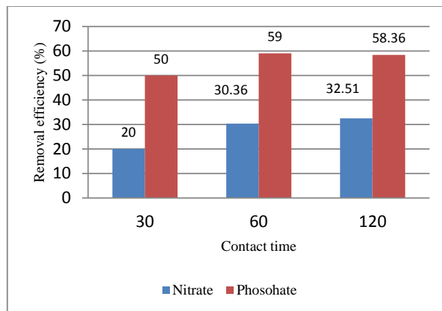
Figure 7a. Effect of contact time on the removal of nitrate and phosphate at adsorbent dose 1 gr/l and mixing speed 100 rpm
