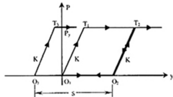
(b) : Deformation-Force Curve of TID
