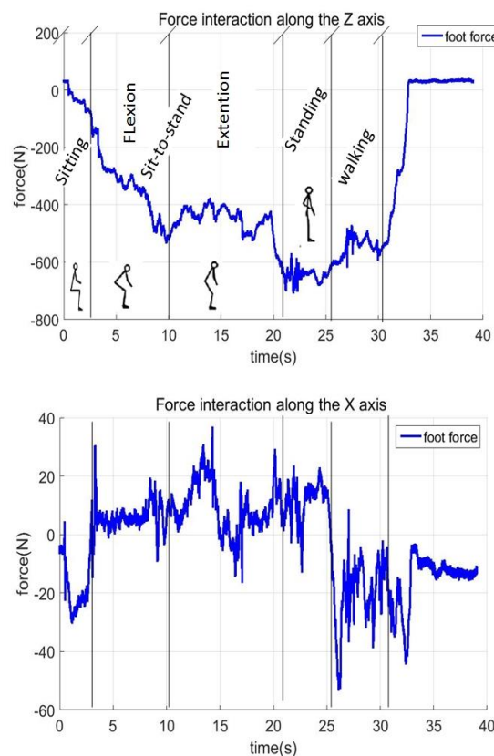
Fig. 10 Vertical and Propulsion reaction forces in STS transfer and walk using S-AD
