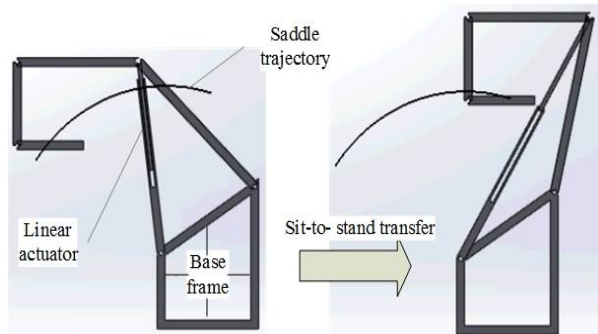
Fig. 4 4-link mechanism in accordance with the trajectory of the shoulder
