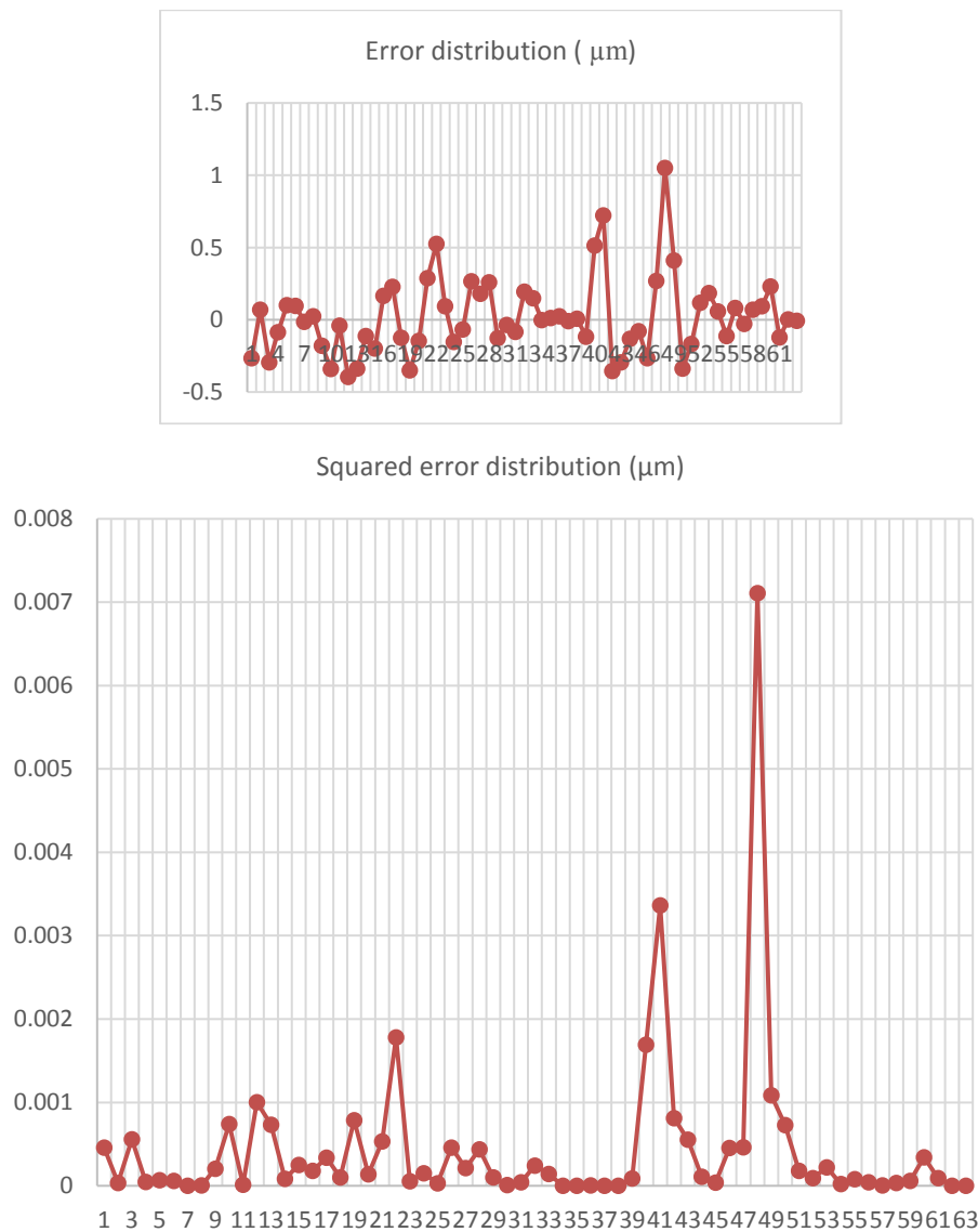
Fig. 4 Distribution of the errors and squared errors for ANN online prediction model
