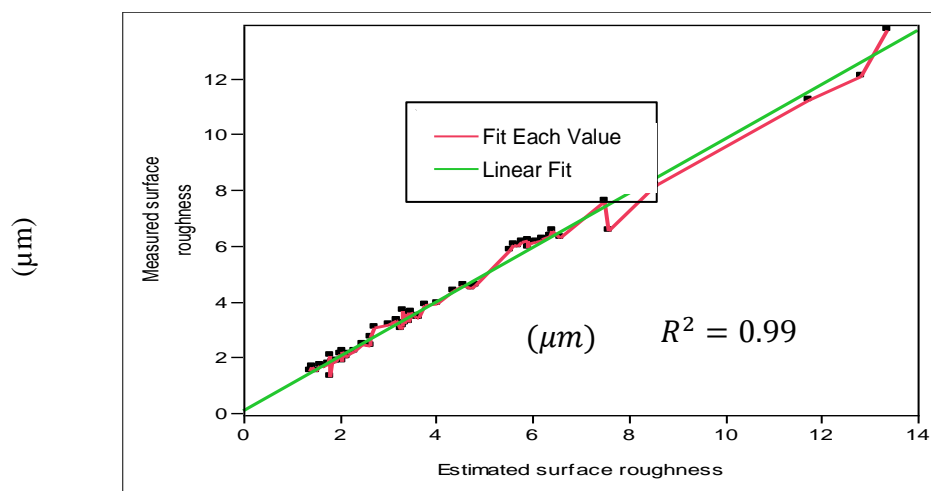
Fig. 5 Comparison of estimated and measured results
