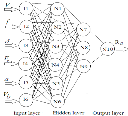
Fig. 2 The designed ANN model
