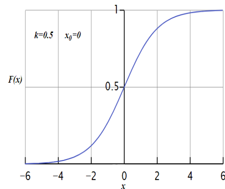
Fig. 3 Logistic activation function diagram for k=0.5 and x_0 = 0
