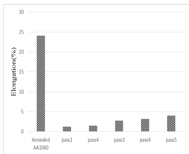
Fig. 5 Variations of the elongation value of AA1060/Al 2 O 3 composites with the Warm-ARB passes
