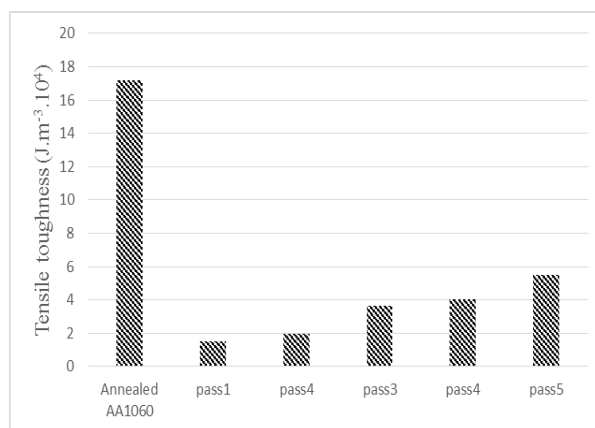
Fig. 6 Variations of tensile toughness with the Warm-ARB passes
