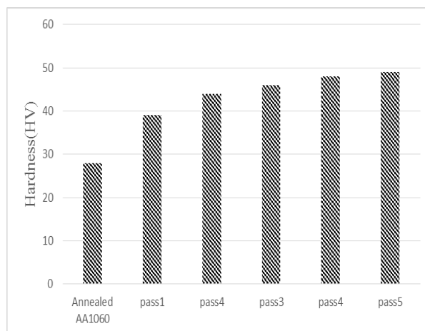
Fig. 7 Variations of Average micro-hardness values with the Warm-ARB passes
