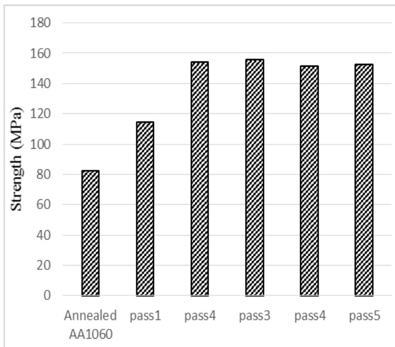
Fig. 4 Variations of the strength value of AA1060/ Al 2 O 3 composites with the Warm-ARB passes
