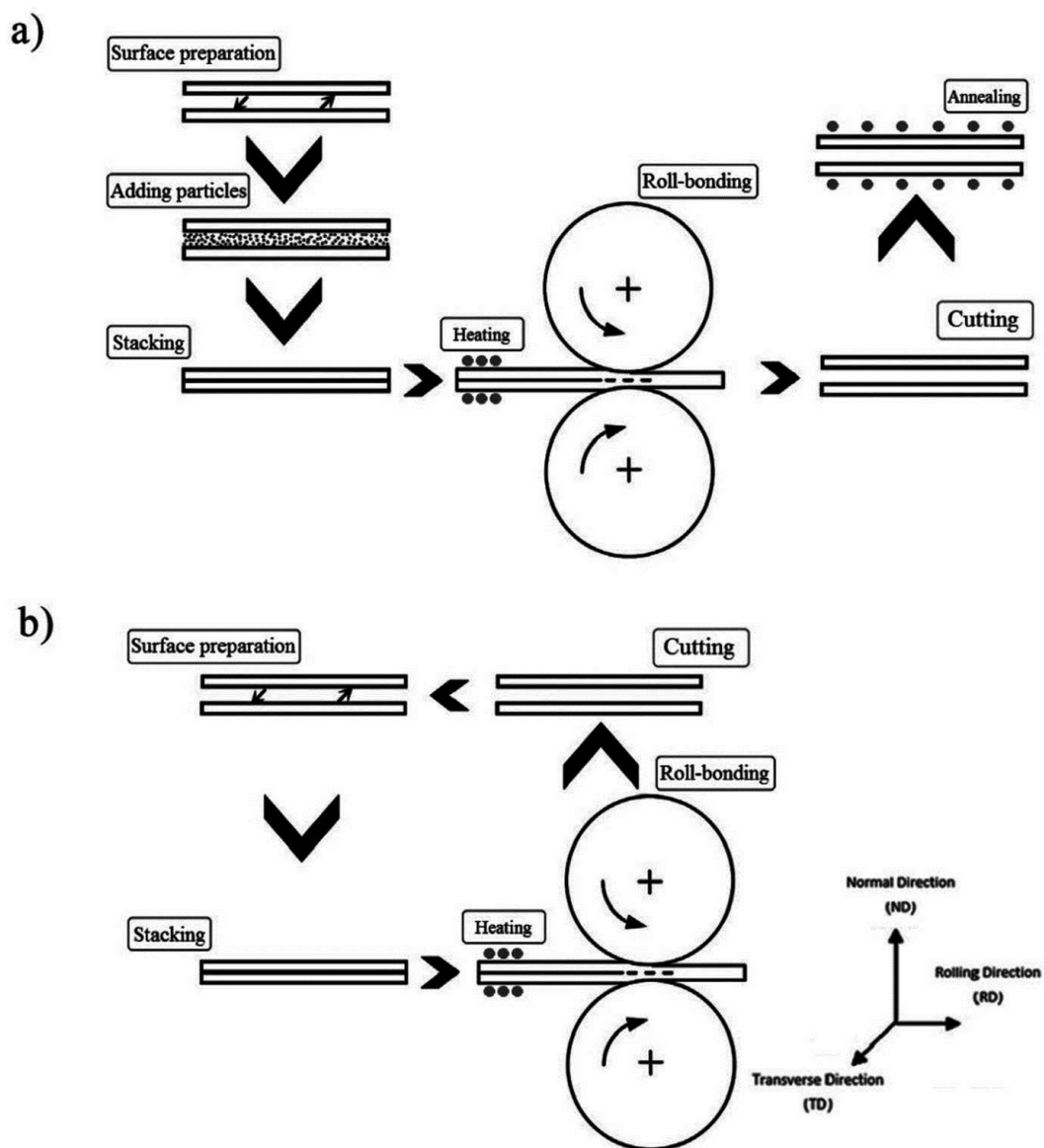
Fig. 1 Schematic illustration of the production process of the AA1060/ Al_2O_3 composite sheet (a): primary cycle (cycle#0) and (b): main cycles
