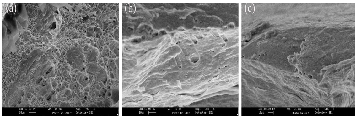
Fig. 7 The fracture surfaces after the tensile test for (a) primary composite (pass #0) and composite with (b) three and (c) five Warm-ARB passes after the tensile test
