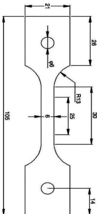
Fig. 2 Orientation of the tensile test specimens (ASTM-E8M), [18]
