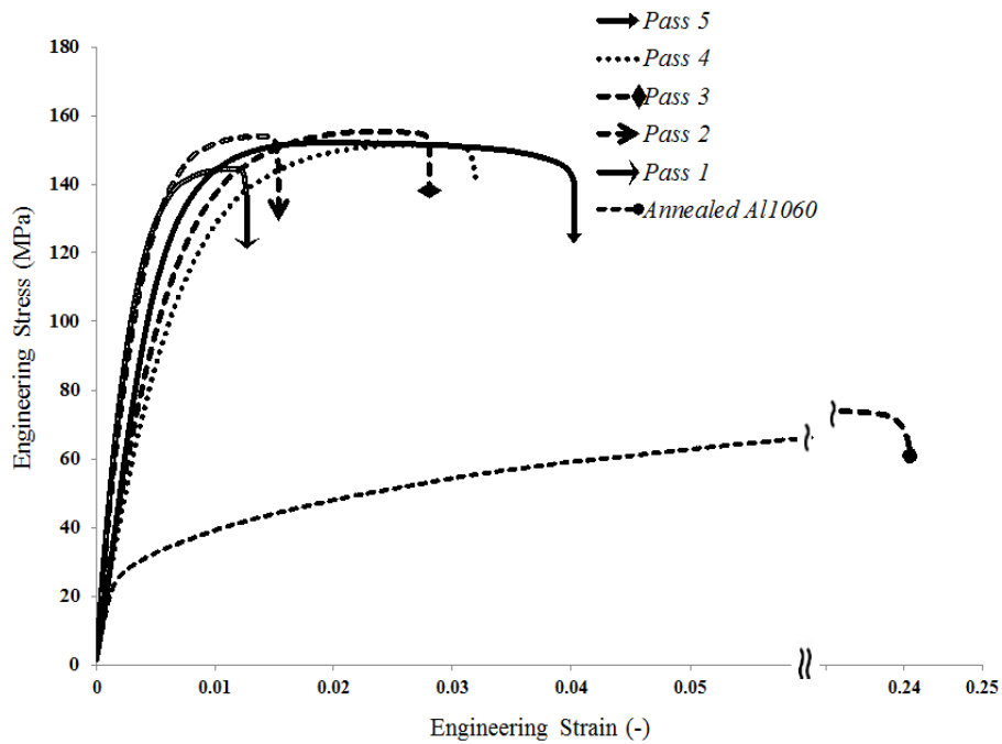
Fig. 3 Engineering stress-strain tensile test curves for Al/ Al 2 O 3 composites before and after Warm-ARB
