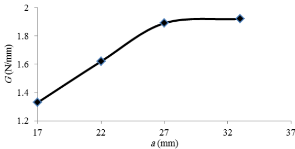
Fig.13 Compliance-crack length diagram, its equation and derivative equation for specimen 10.
