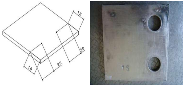
Fig.7 Marking and drilling of specimens.
