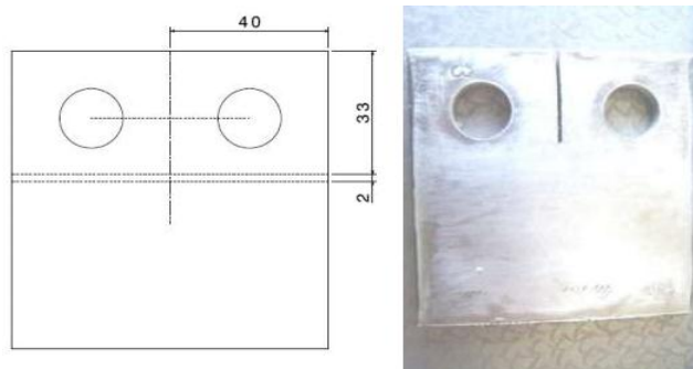
Fig.8 Marking and crack creating on specimens.
