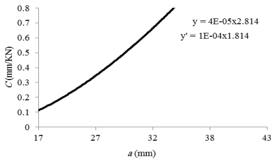
Fig.12 Crack propagating energy-crack length diagram for specimen 11.
