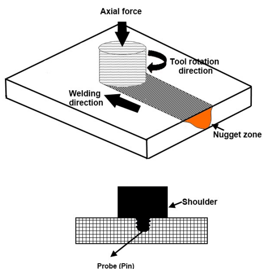
Fig. 1 Schematic drawing of friction stir welding process
