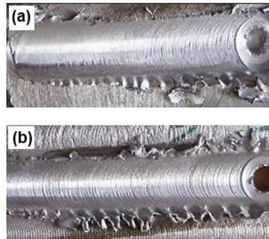
Fig. 3 Surface appearances of 6061+15% \text{Al}_2\text{O}_3\text{p} composite joined by FSW as a function of tool rotational speed, (a) 630 r/min and (b) 1250 r/min
