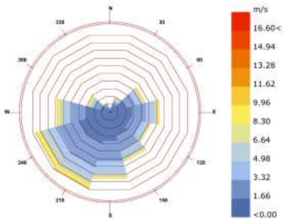
Figure 3.1: Mashhad Wind-Rose Chart for Annual Wind Speed and Direction (Based on Ladybug Software Analysis)
