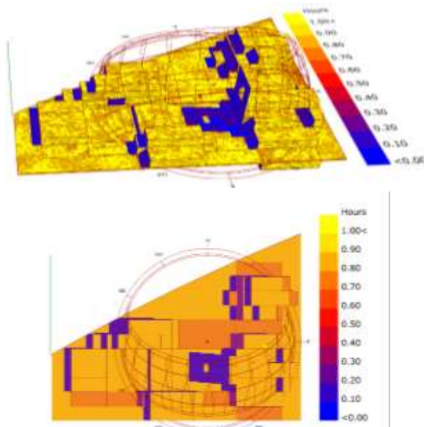
Figure 5.2: Simulation of the Amount of Radiation and Solar Energy on the Surfaces of the Building According to the Adjacency, Shape, and Direction of the Building in Summer at 15 p.m. in the Final Proposal (Based on Ladybug Software Analysis)
