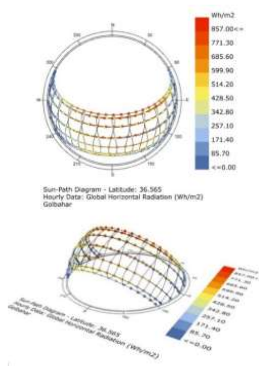
Figure 3.10: The Annual Solar Conveyer Chart of Golbahar City (Based on Climate Software Analysis)
