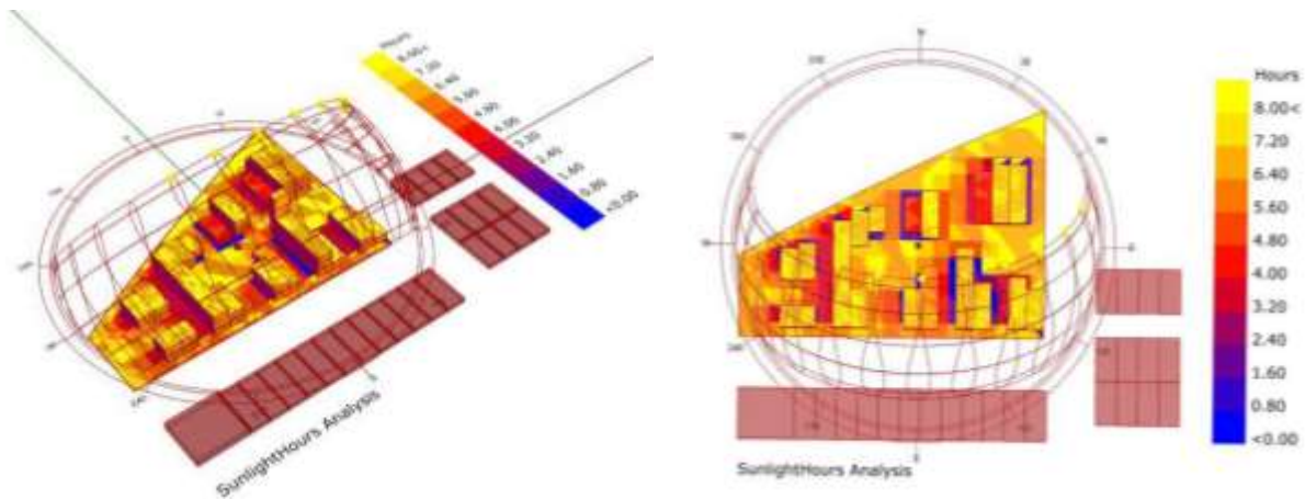
Figure 3.14: The Summer Sunlight Chart (Based on Climate Software Analysis)
