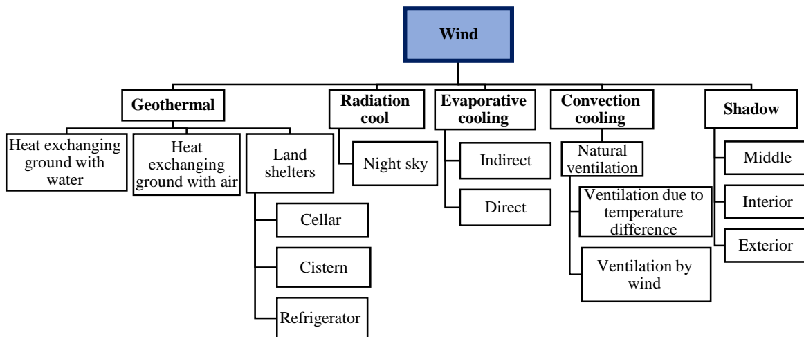
Chart 2.2: Supplying the Building Thermal Requirements out of Wind
