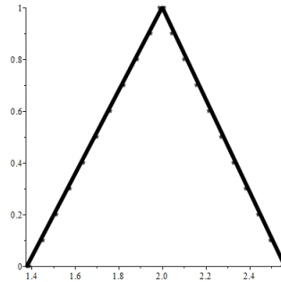
Figure 1: The approximation(Dots) and Exact(Line) of fuzzy solution at t = 2 .
