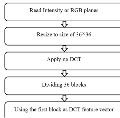
Fig. 3. Generating DCT feature.
