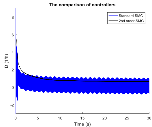
Fig. 18. The comparison of D designed by Standard SMC and 2 nd order SMC
