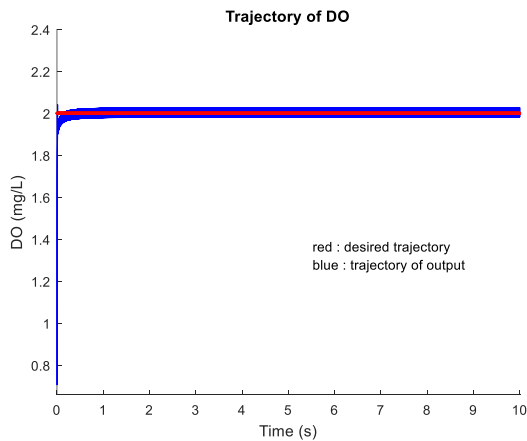
Fig. 10. Trajectory of DO by Standard SMC.
