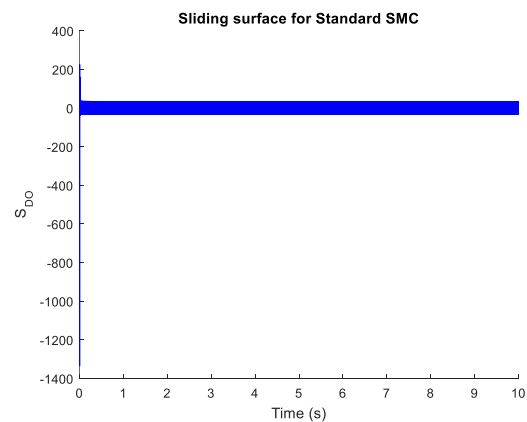
Fig. 4. Sliding surface to control DO by Standard SMC.
