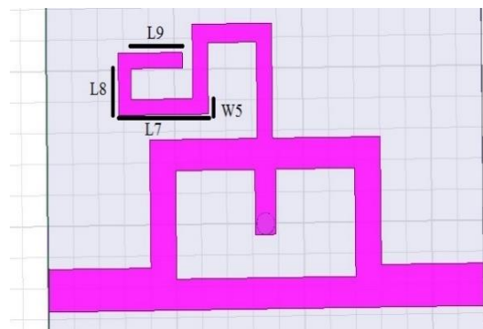
Fig. 8. Simulated structure of the third proposed filter with HFSS software.
