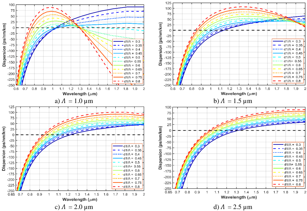
Fig. 5. Graph of the dispersion characteristic D of the hexagonal lattice structure filled by \text{CHCl}_3 .
