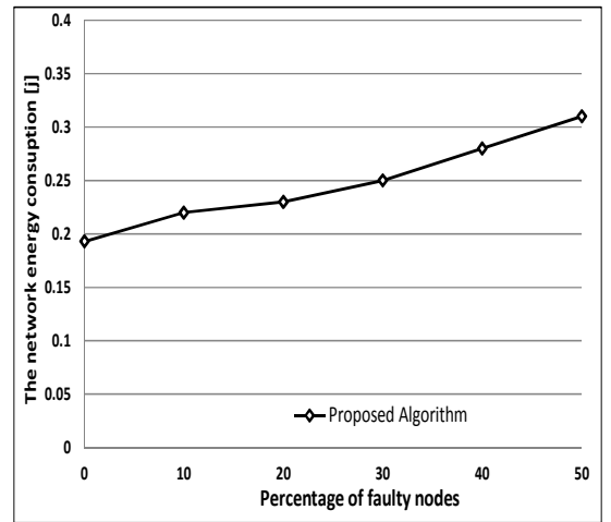
Figure 5. The network energy consumption vs. percentage of faulty nodes.
