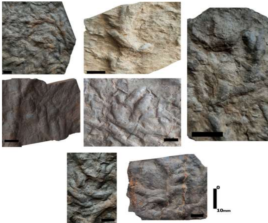
Figure 13. Ichnofossils Treptichnus pedum
