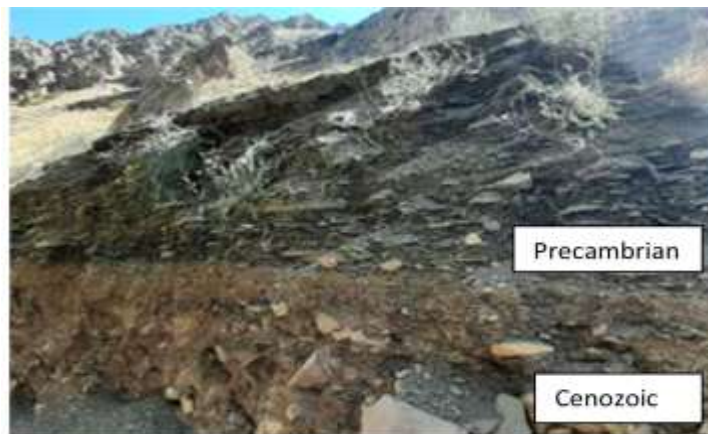
Figure 12. Contact Lower Shale member (Precambrian) with Cenozioc, View of South eastside
